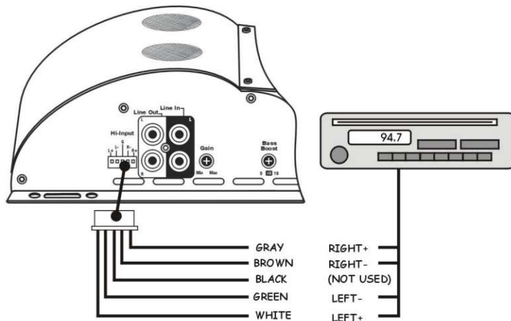
TWO CHANNEL CONNECTIONS: FLOATING GROUND RADIO (MOST COMMON TYPE)
